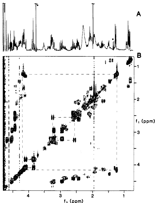
FIGURE 5: Aliphatic region of 300-MHz 1 H NMR spectra of gastrin in 2 H 2 O at 25 °C. (A) One-dimensional spectrum of 0.6 mM gastrin, pH 6.4. Time-domain data, consisting of 1500 transients acquired in 8192 addresses, were multiplied by a Lorentz-Gauss window function and zero filled to 16384 addresses prior to Fourier transformation. Resonances from impurities are marked with asterisks. (B) Contour plot of two-dimensional homonuclear correlated (COSY) spectrum of 3.0 mM gastrin at pH 6.5. Spectral conditions are given under Materials and Methods. Spin-spin coupling connectivities are shown for Gly-2 α-CH 2 in the cis and trans forms and for Ala-11 α-CH-β-CH 3 .
